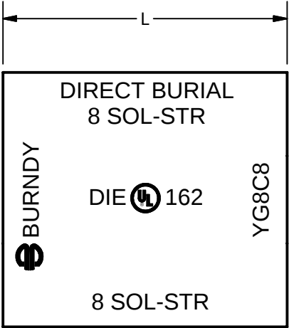
TYPICAL LETTERING
